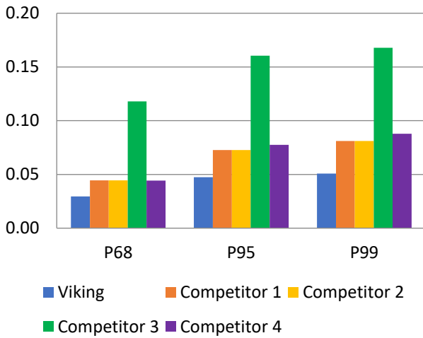
Vertical Position Error (m)
